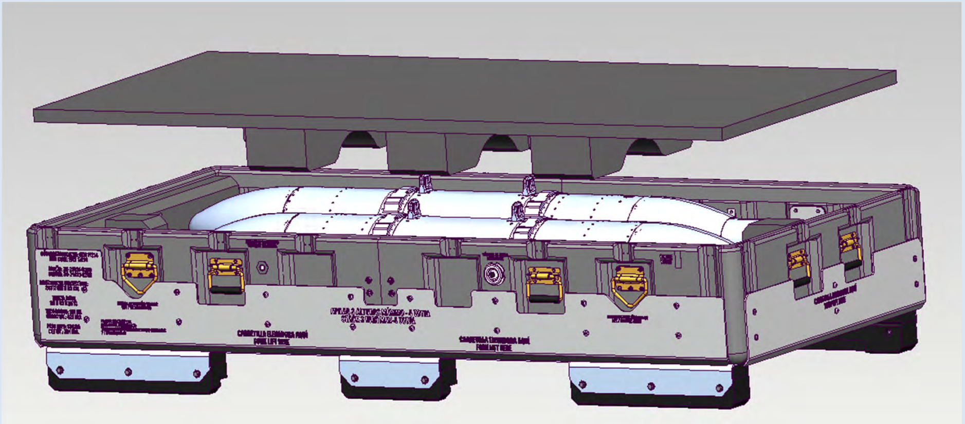
SHOWN WITH LID CUSHION LID CUSHION LOWERS ON GENERATORS AND SECURES THEM FOR TRANSIT
